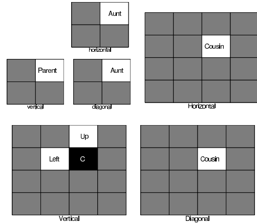
Figure 6: Relations Between Wavelet Coefficients
