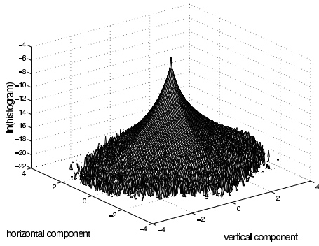
Figure 7: Mesh Plot of the \ln(\text{Joint Histogram}) of Horizontal Component and its Vertical Cousin
