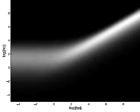
Figure 11: The conditional histogram H(\ln|hc| | \ln|hp|) calculated from our model. Bright parts mean high values
