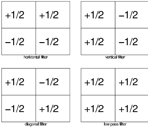
Figure 5: Haar Filters
