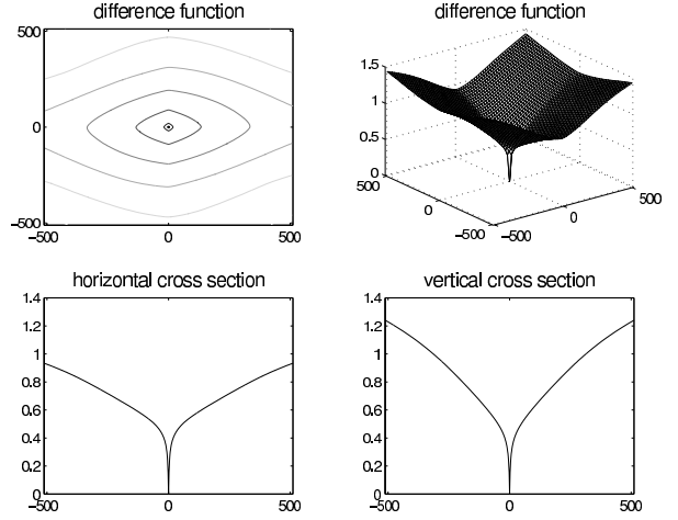
Figure 12: Difference Function
