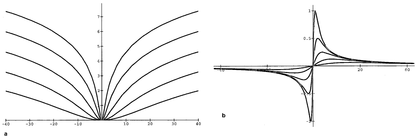
FIG. 9. Graduated Non-Convexity. \rho(x, \sigma) and \psi(x, \sigma) plotted for thresholds \tau \in \{16, 8, 4, 2, 1\} . (a) Error measure \rho(x, \sigma) . (b) Influence, \psi(x, \sigma) .
