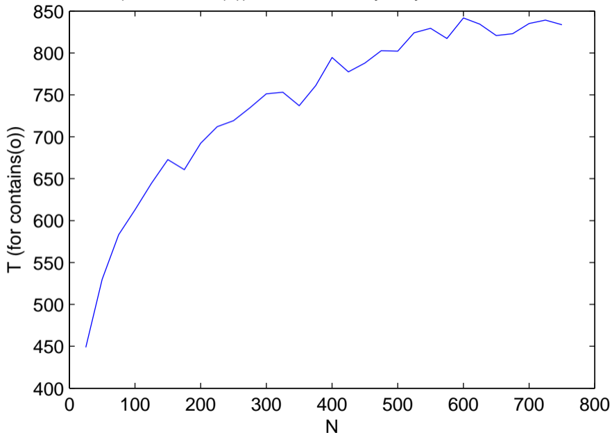
T (for contains(o)) versus N for Mystery Data Structure 0
